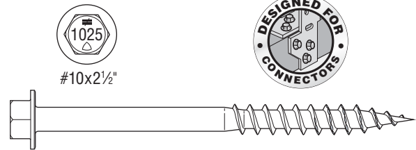
#10 x 2 1/2" Strong-Drive® SD Structural-Connector Screw U.S. Patent 7,101,133
