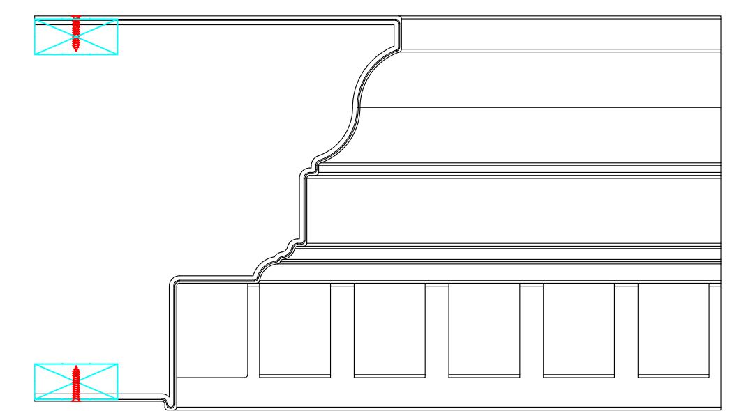
ELEVATION OF CR-115X8 IN CORNER SCALE 1:1
