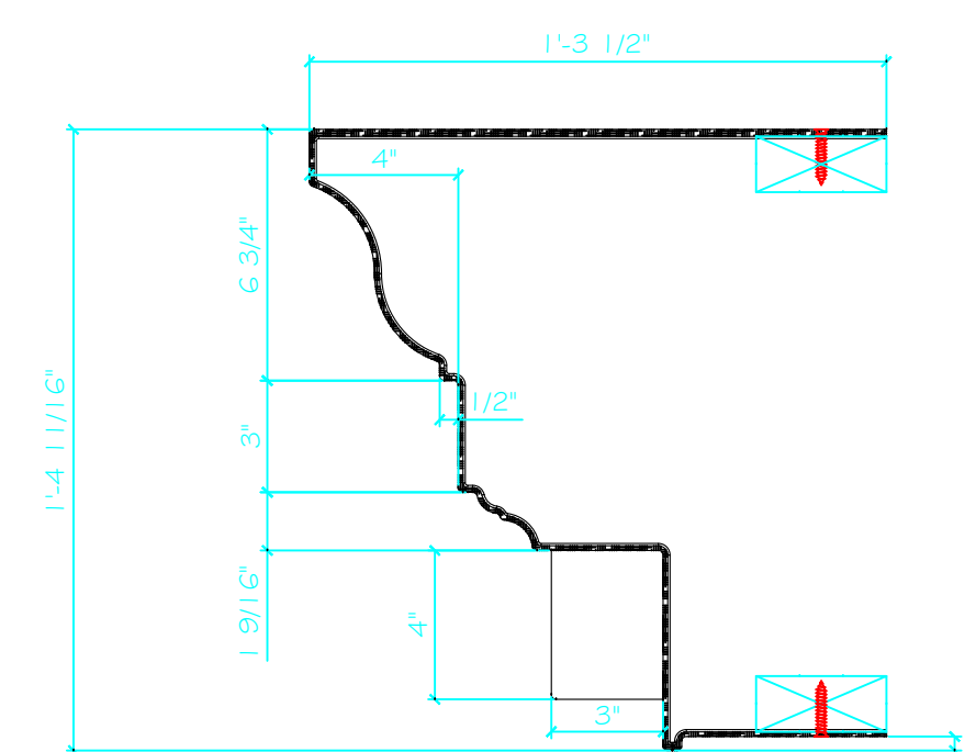
SECTION THRU CR-115X8 SCALE 1:1
