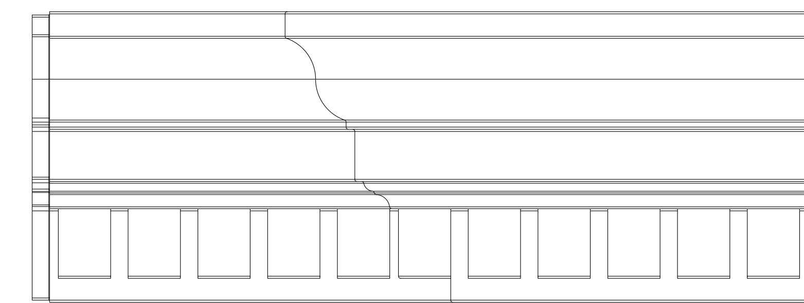
ELEVATION OF CR-115X8 FROM OUT CORNER SCALE 1:1
