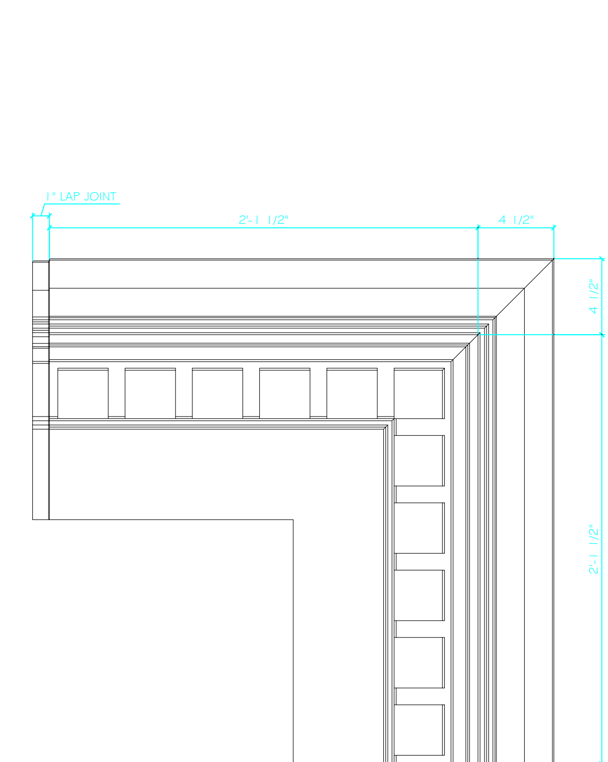
CR-115X8 OUTFROM BELOW SCALE 1:1
