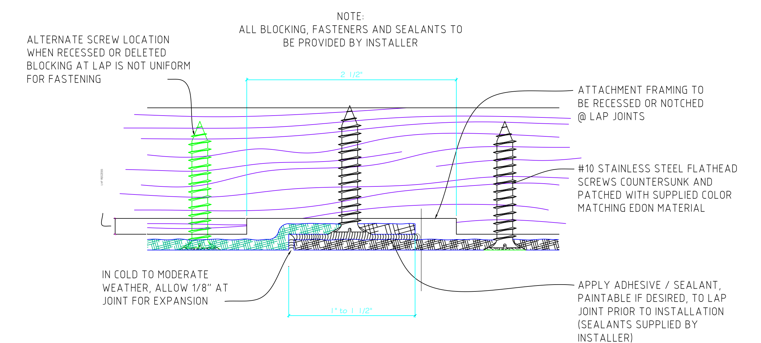
B 1 LAP JOINT DETAIL FULL SCALE
