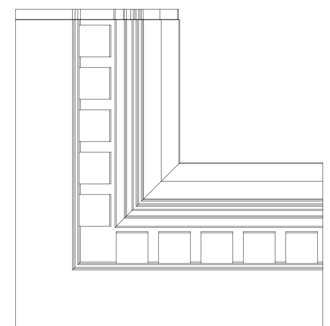
CR-115X8 IN CORNER FROM BELOW SCALE 1:1
