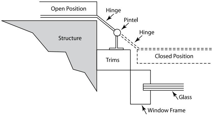
Recessed
