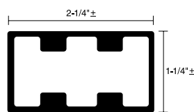
Wall Thickness 9/32" ±
