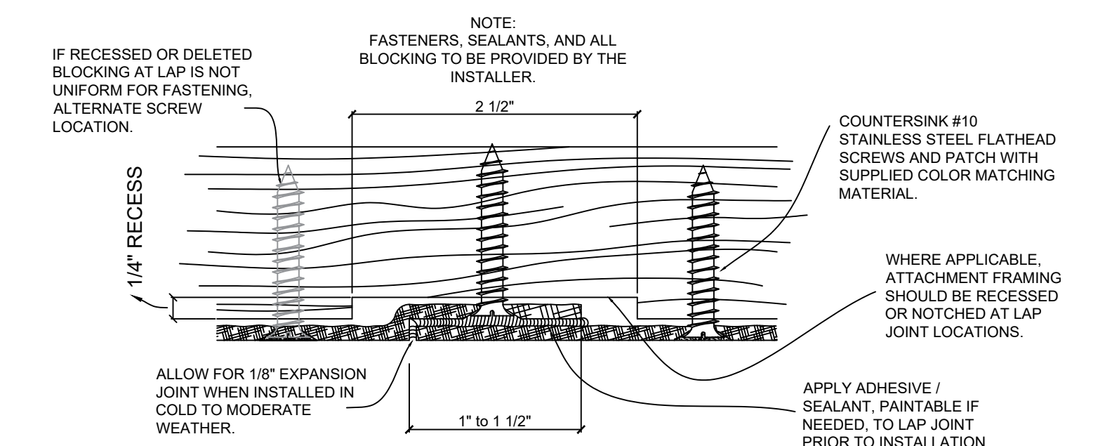
11 Typical Lap Joint Detail Not to Scale
